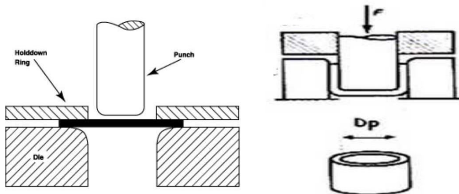
Fig.1 Deep drawing process
